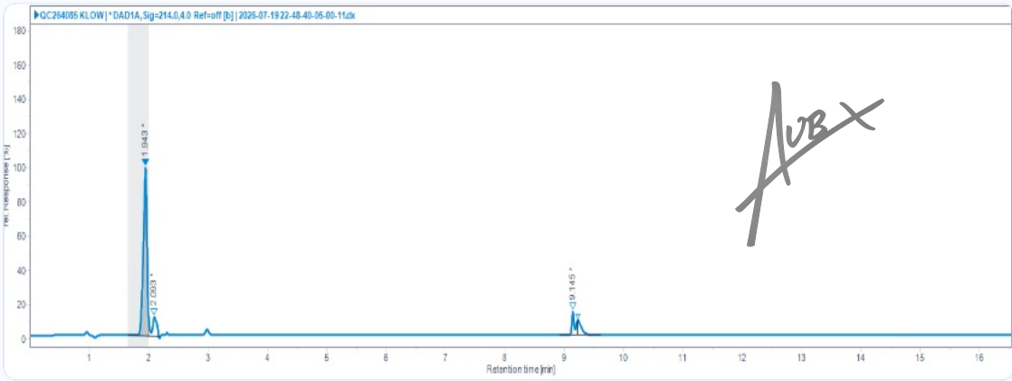
HPLC Chromatogram (Retention Time: 1.940, 2.319, 9.146, 9.230 min)
